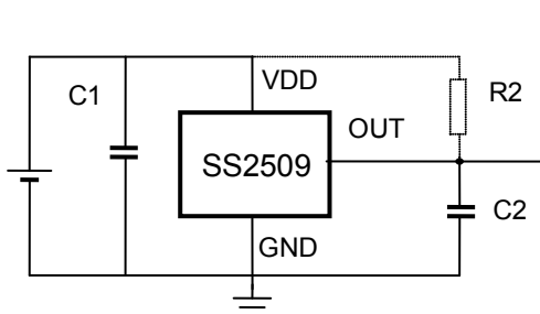
Typical Three-Wire Application Circuit
